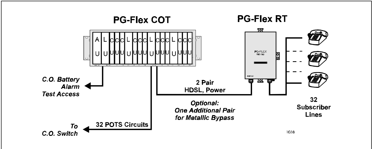
Figure 2. Typical PG-Flex Configuration.
