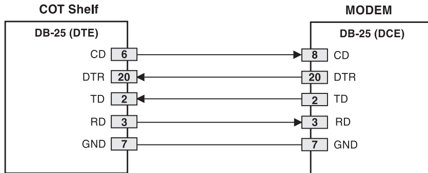
Figure 4. Modem Connection for FCS-717 Backplane
