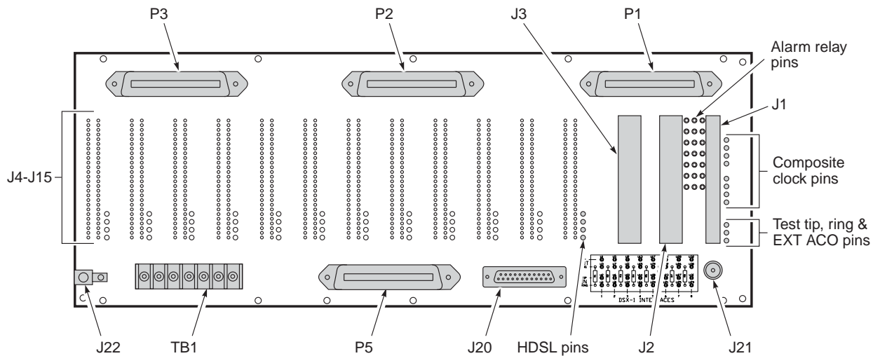
Figure 2. PCS-718 Shelf Backplane
