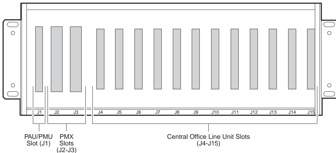
Figure 1. Front View of the PCS-718 COT Shelf
