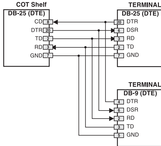
Figure 5. Null Modem Connection for FCS-717 Backplane
