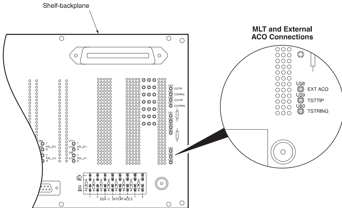
Figure 12 External ACO Wire-Wrap Connections
