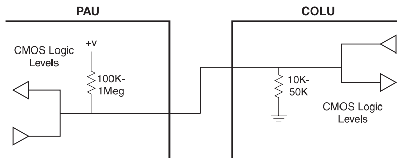
Figure 3 Communication Line Between PAU/PMU and COLU
