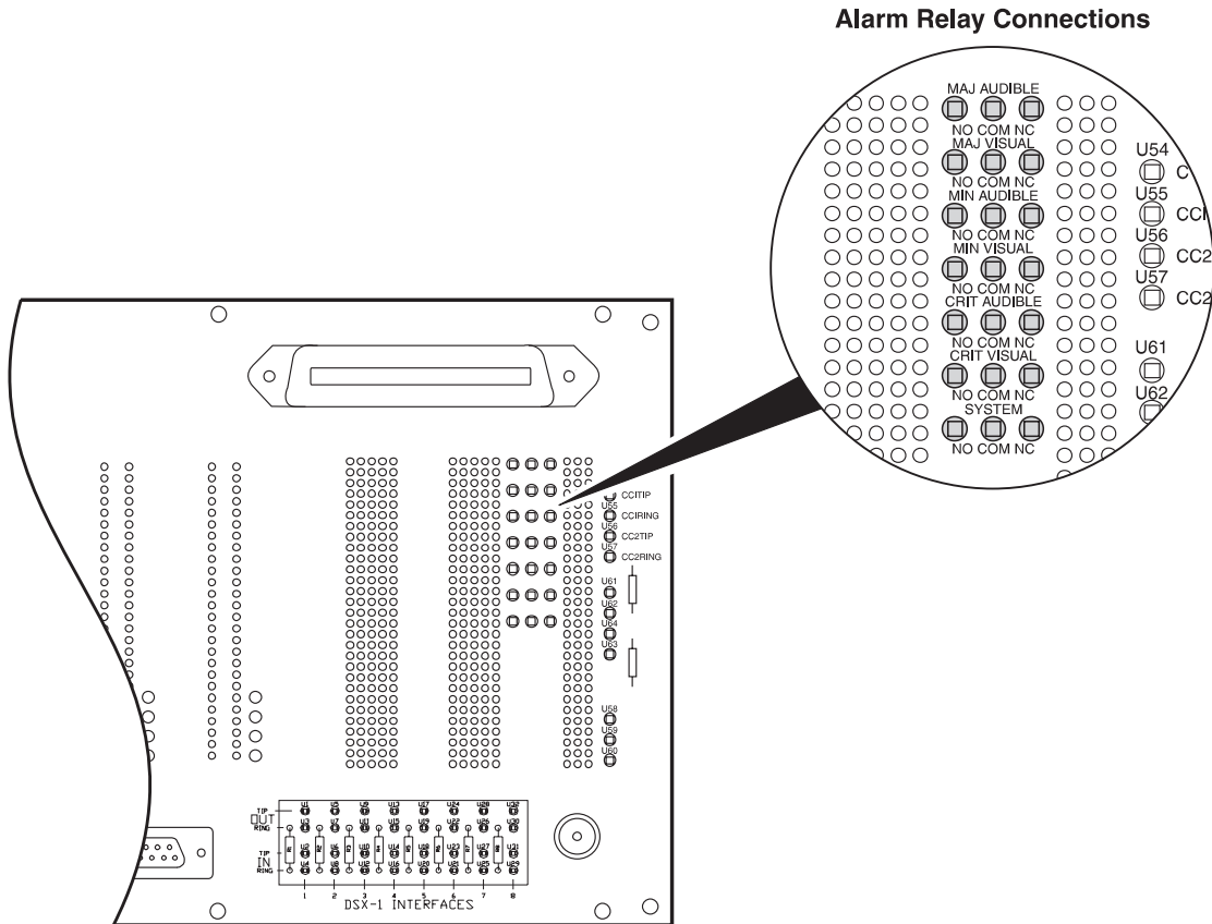
Figure 9 Alarm Relay Wire-Wrap Field
