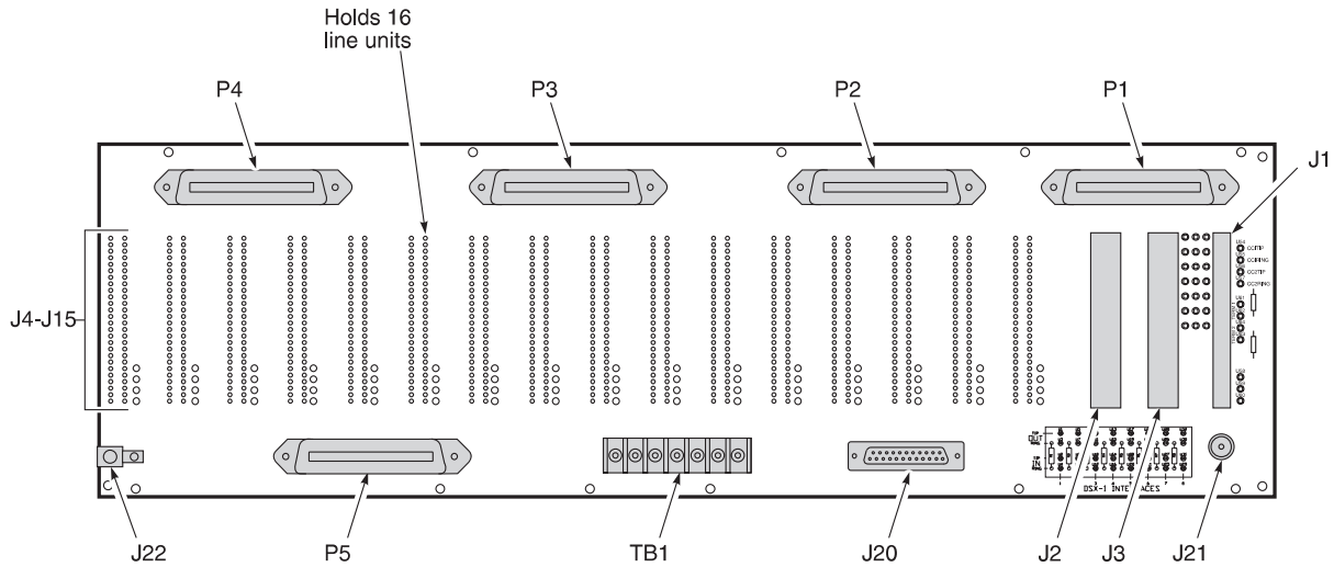
Figure 4 PCS-719 Shelf Backplane
