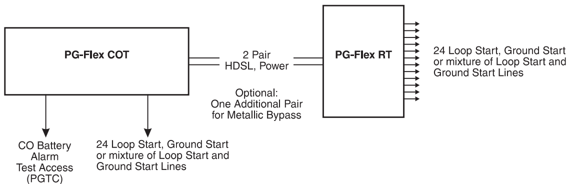
Figure 2. Typical System with Loop Start and Ground Start Capabilities
