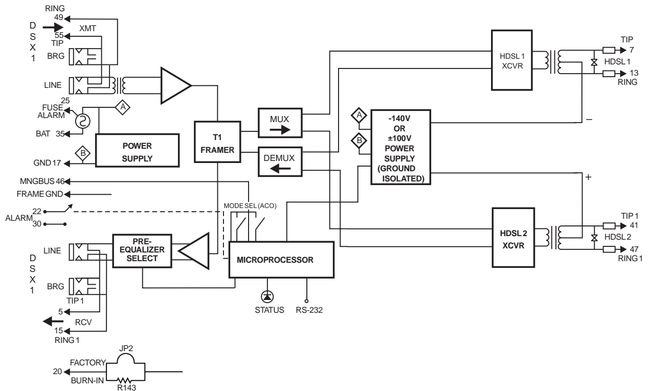
Figure 23. HLU-431 Block Diagram
