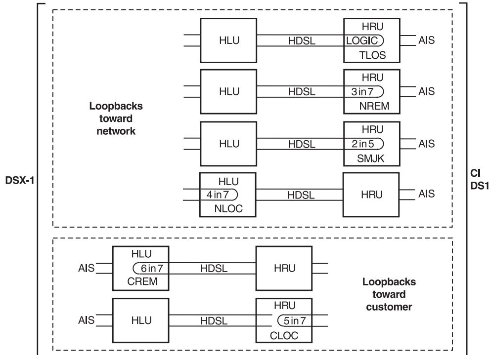
Figure 21. HLU-431 Non-Doubler Loopback Configurations
