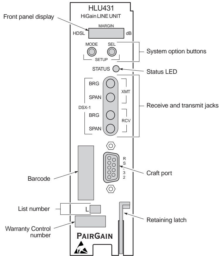
Figure 1. HLU-431 List 1E Front Panel
