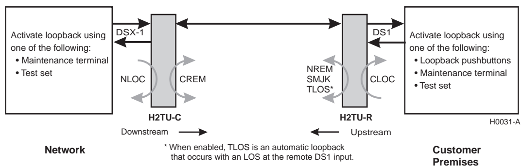
Figure 28. Loopback Summary
