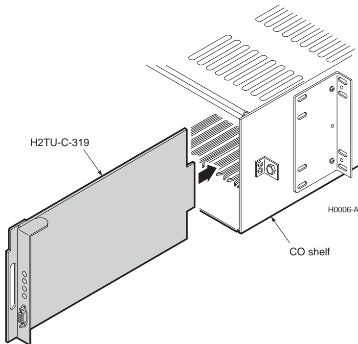
Figure 2. Installing an H2TU-C into a Shelf
