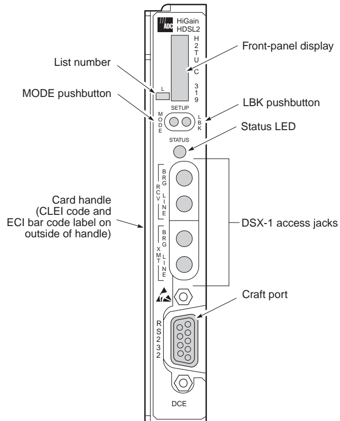
Figure 1. H2TU-C-319 List 3F Front Panel
