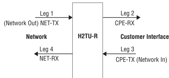
Figure 11. Sectionalized Analysis of the DS1 Interface
