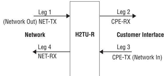
Figure 28. Sectionalized Analysis of the DS1 Interface
