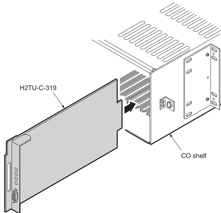
Figure 2. Installing the H2TU-C-319 List 3F into a Shelf
