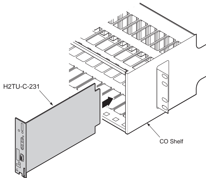
Figure 2. Installing the H2TU-C-231 List 2F into a Shelf
