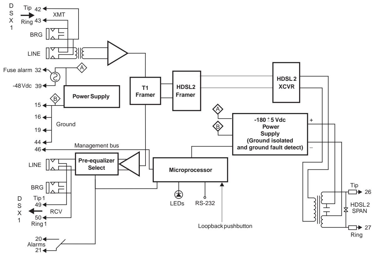
Figure 36. H2TU-C-231 List 2F Block Diagram
