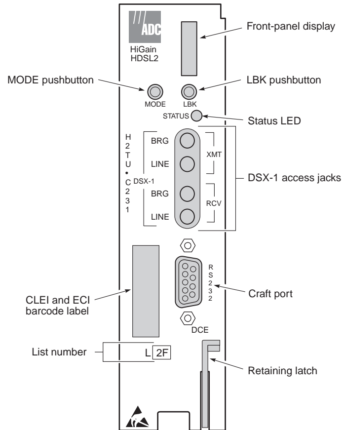
Figure 1. H2TU-C-231 List 2F Front Panel
