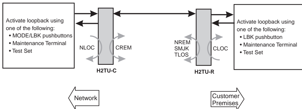
Figure 32. Loopback Summary
