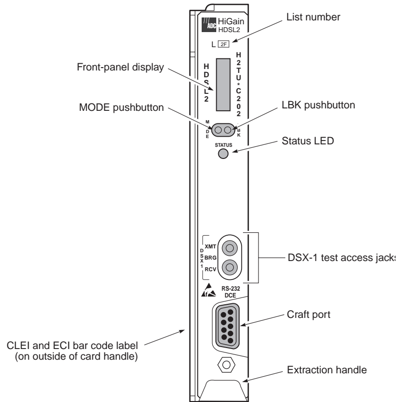
Figure 1. H2TU-C-202 List 2F Front Panel
