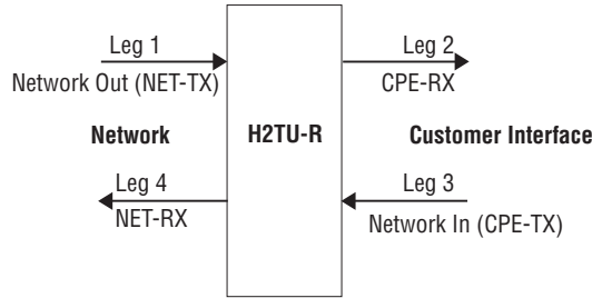
Figure 29. Sectionalized Events
