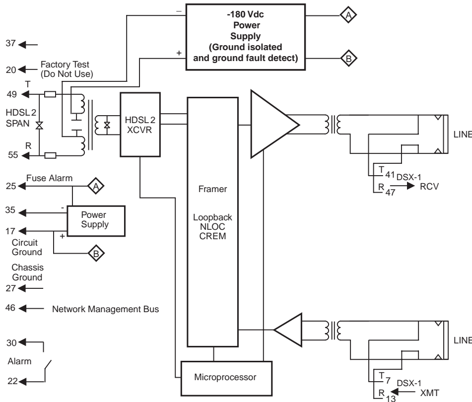
Figure 37. H2TU-C-202 List 2F Block Diagram
