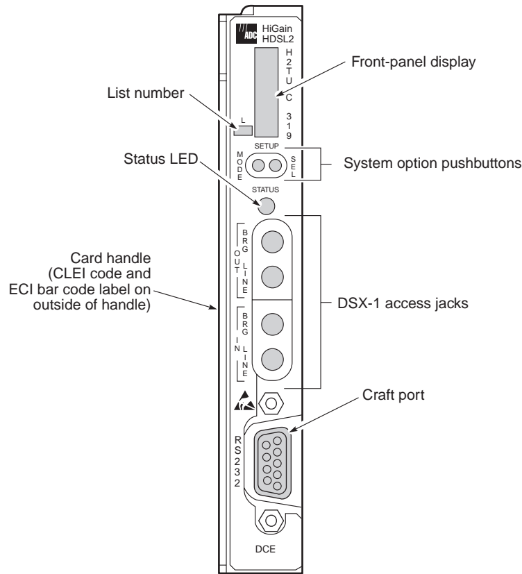
Figure 2. H2TU-C-319 List 1E Front Panel
