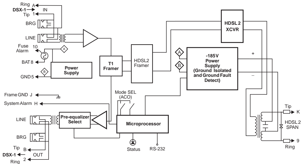
Figure 32. H2TU-C-319 List 1E Block Diagram
