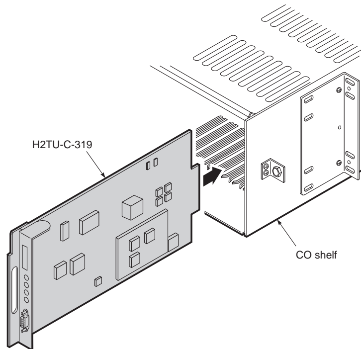
Figure 3. Installing the H2TU-C-319 List 1E into a Shelf
